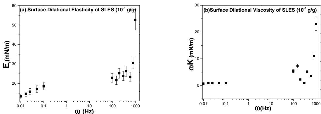
Fig: (a) Real and (b) Imaginary parts of Surface Dilational Elasticity as a function of frequency
