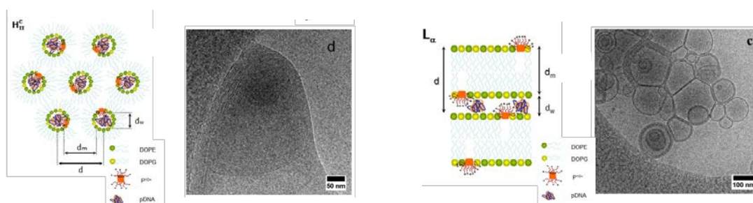
Figure 1. Schematic drawing of Hexagonal ( H_{II}^C ) and lamellar ( L_a ) phases of lyotropic liquid crystals found in DOPG/DOPE- \text{P}^{10+} -pDNA lipoplexes
