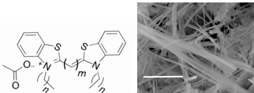
Figure 1: Chemical structure of studied thiocyanine dyes and example of derived silicatropic material
