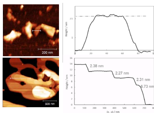
Figure 1. AFM micrographs and height profile of: (top) nominal monolayer and (bottom) terraces of a graphene flake.
