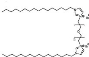
Figure 1. Structure of GCLs series: (C_{16}Im)_2(C_2H_4O)_n C_2H_4 (with n = 3 )
